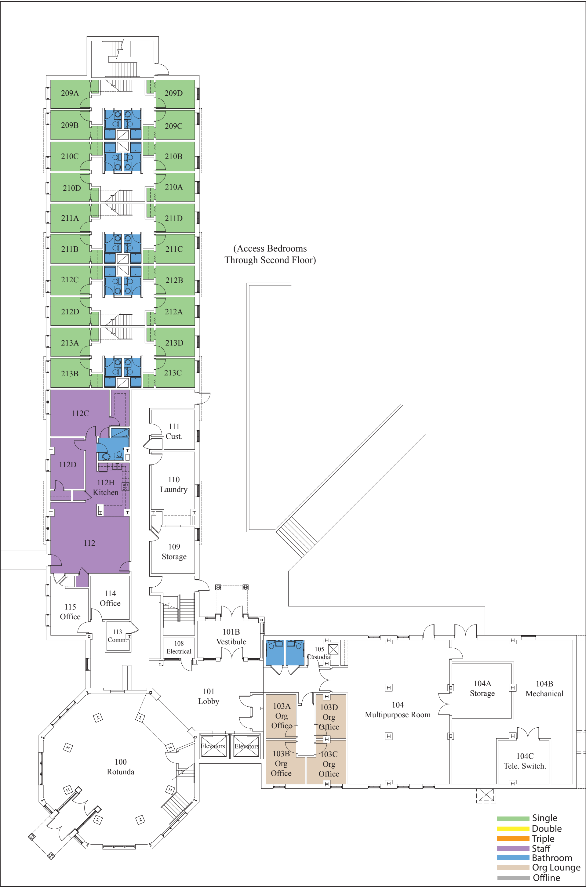
Polo Residence Hall First Floor Plan
