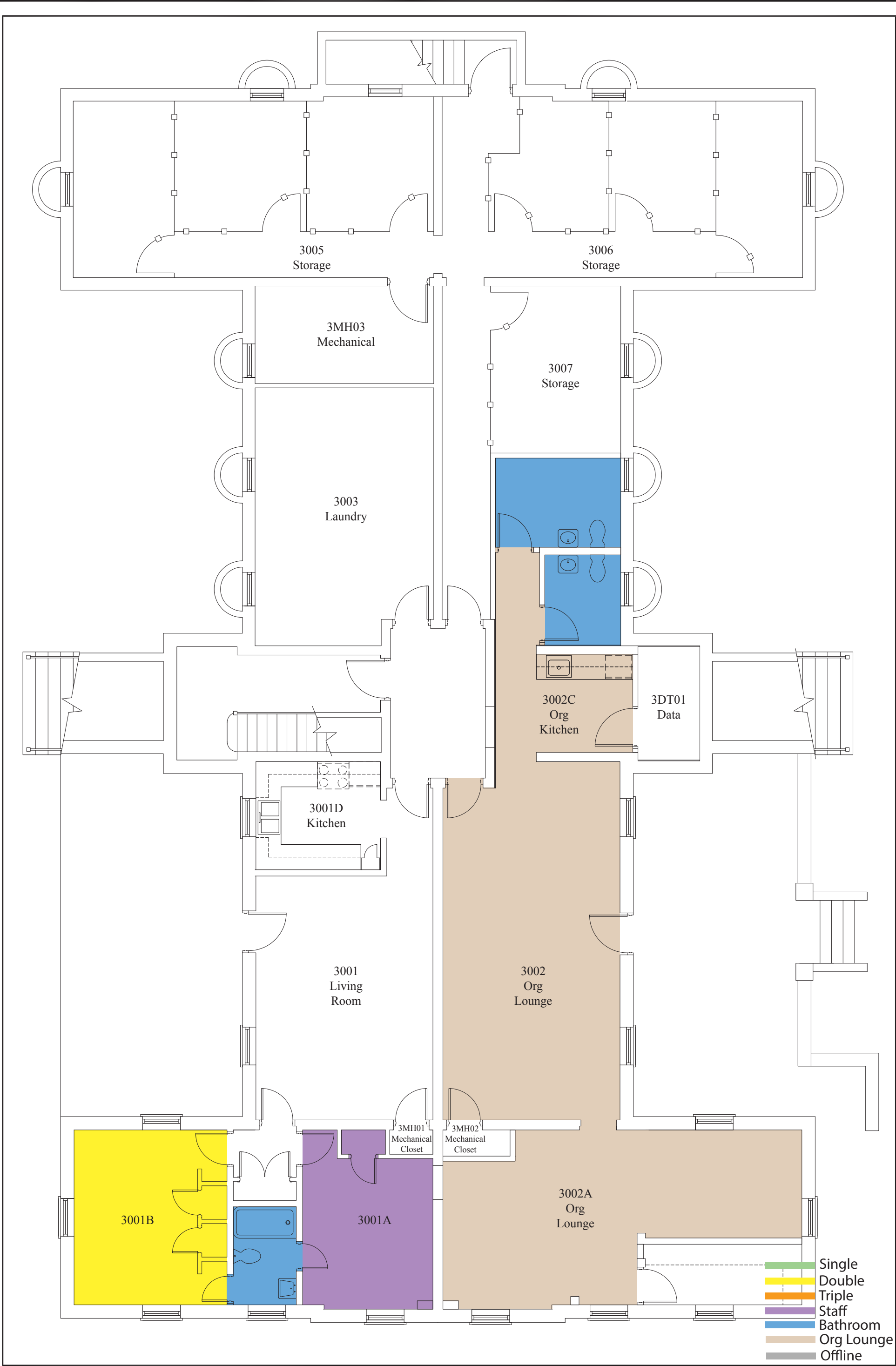
North Campus Apartment Building 3 Ground Floor Plan
