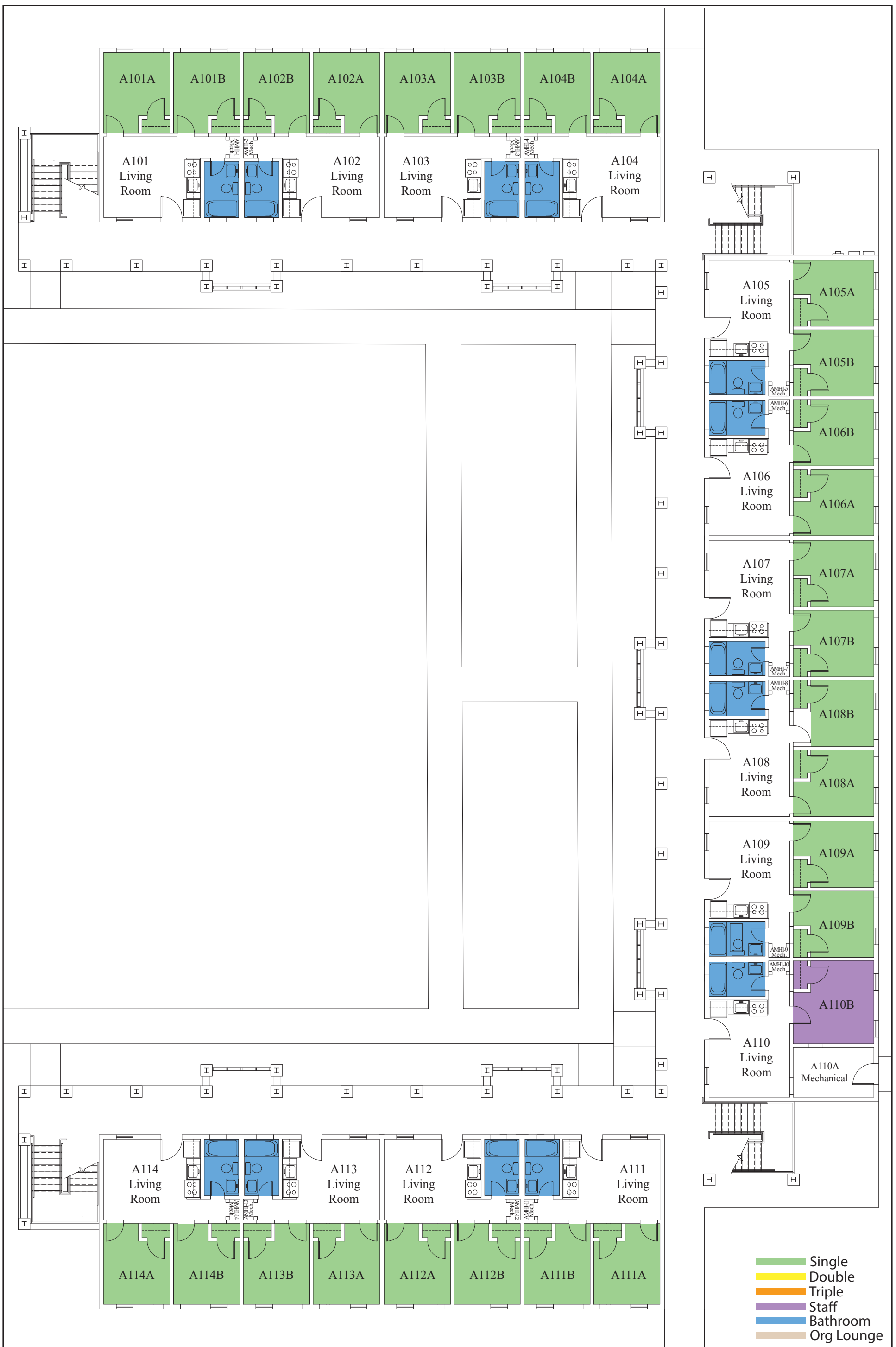
Student Apartments Bldg. A First Floor Plan
